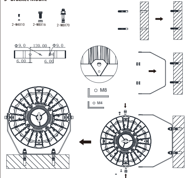
3- Bracket Mount
